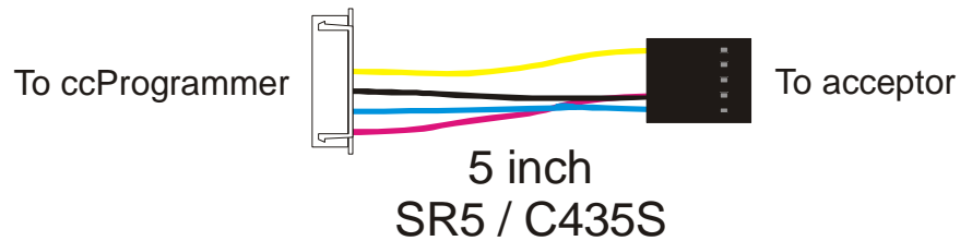
Figure 3: ccProgrammer 3 inch acceptor cable
