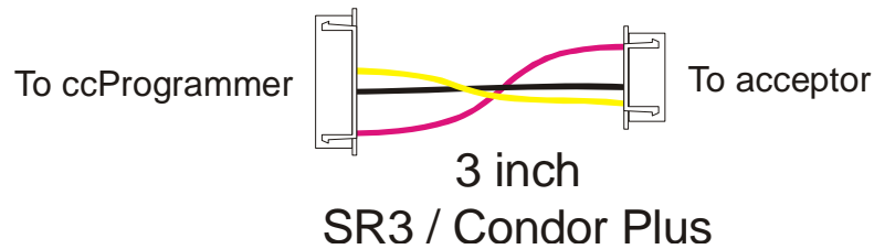
Figure 4: ccProgrammer serial comms cable
